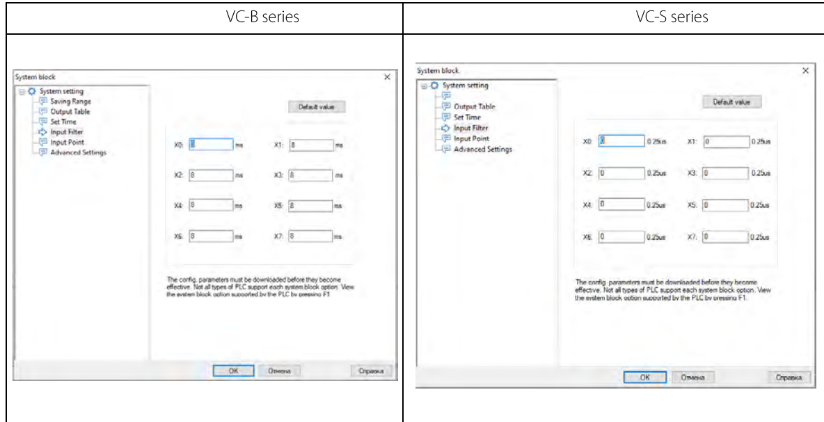
Figure 2-4 set input filter
