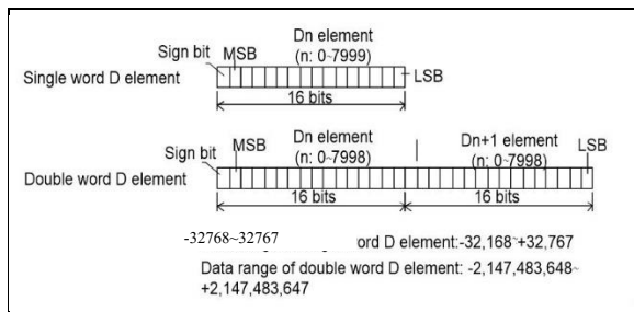
Figure 3-1 D or R element
