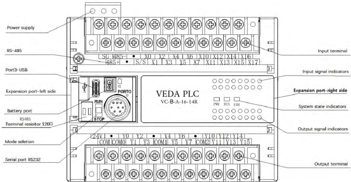
Figure 1-1 VC-B series main module outline structure
