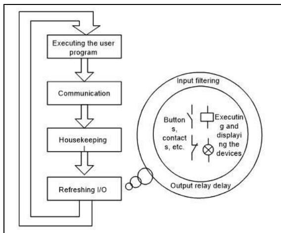
Figure 3-2 I/O refresh principle
