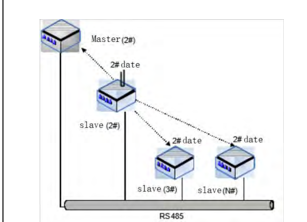
Figure 10-1 Master station broadcast
