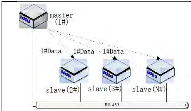
Figure 10-1 Master station broadcast
