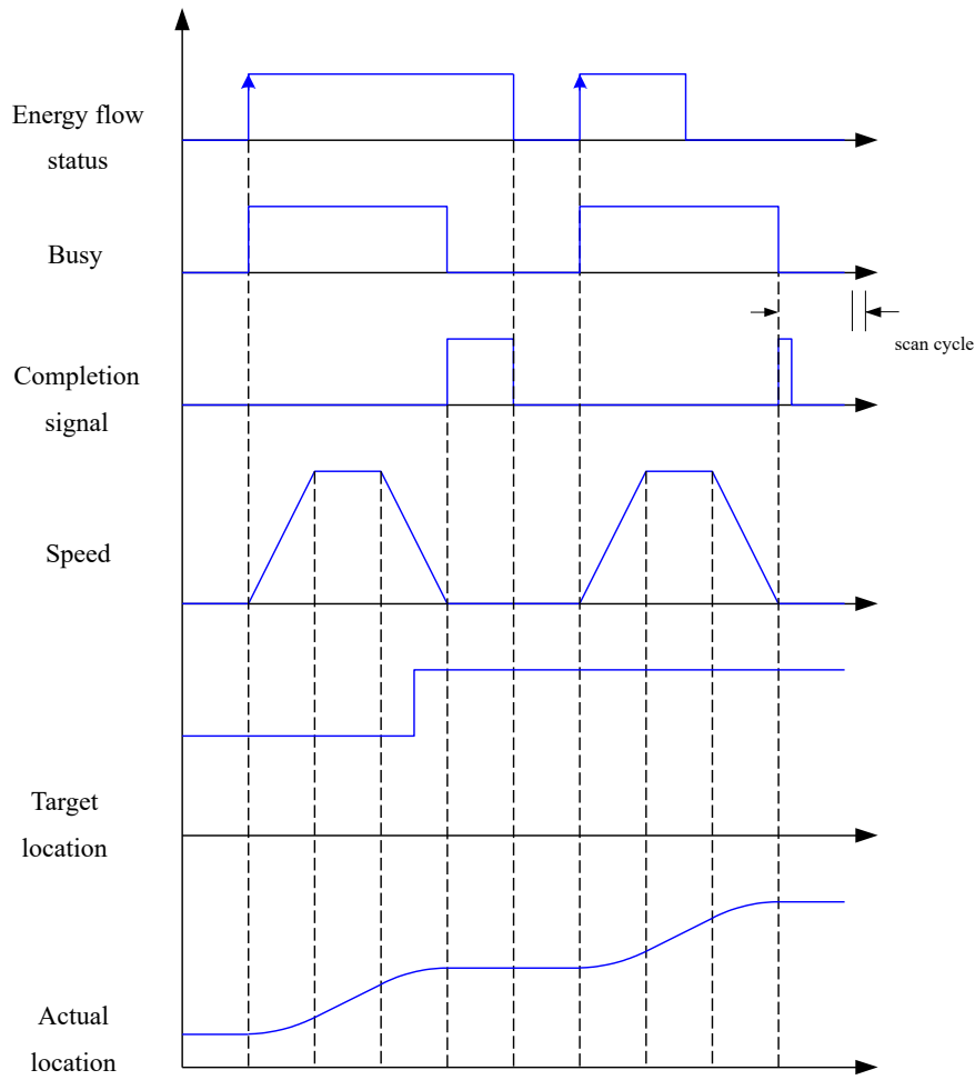
MCMOWEL Timing diagram
